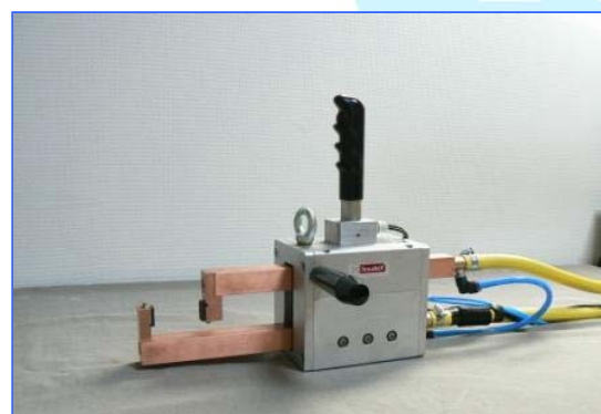
- PIAB micro C welding gun „Parrot“
